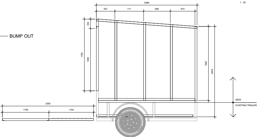
NORTH ELEVATION 1 : 20
