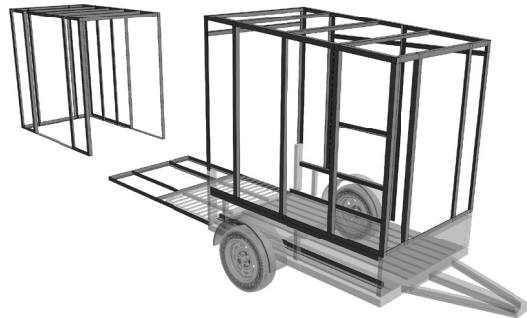
PERSPECTIVE DRAWING
